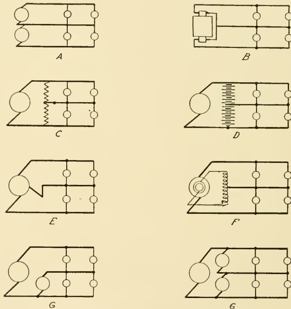
Fig. 13. Diagrams of 3-Wire Generating Methods
